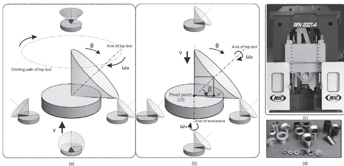
Fig. 1. Kinematic scheme of (a) orbital-type and (b) spin-nutation type rotary forging machine; (c) bespoke MJC RFN 200T-4 machine installed at AFRC and (d) the range of components produced using the machine.
