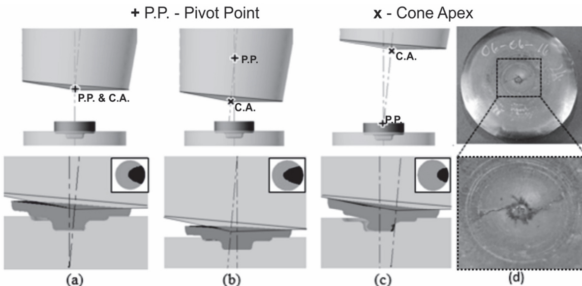
Fig. 2. Positioning of the conical top tool (a) with correct pivot point (PP) alignment, (b) with cone apex (CA) below PP, and (c) CA above PP. Top: alignment before the start of the process; Bottom: Formed geometry at the end of the process; Insert: Contact area between the top tool and workpiece. (d) Enlarged picture of cracks formed when CA is above PP
