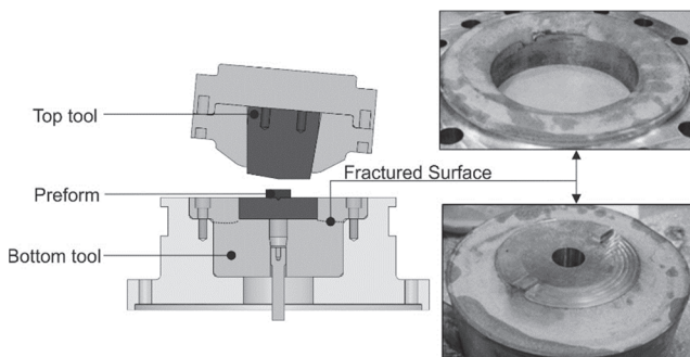
Fig. 8. An example case of a fractured bottom tool caused by the case of high resisting torque in the bottom tool
