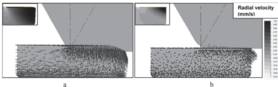
Fig. 7. The radial velocity of points in the material for different bite sizes. Main picture: velocity vectors; Inset: plot of gradients of radial velocity in the part directly under the top tool; (a) bite size of 1 mm/rev, (b) 0.1 mm/rev
