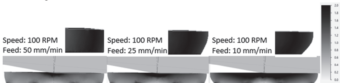
Fig. 6. Side view of the output geometry and plastic strain values obtained at the end of the forming cycle for different speed and feed values.
