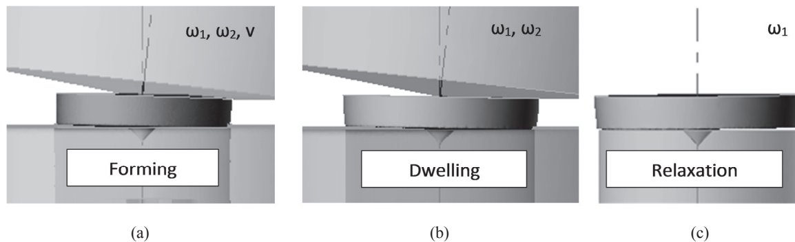
Fig. 3. Modelling of different stages of the forming cycle in rotary forging process: (a) forming step, (b) dwelling step, and (c) relaxation step.
