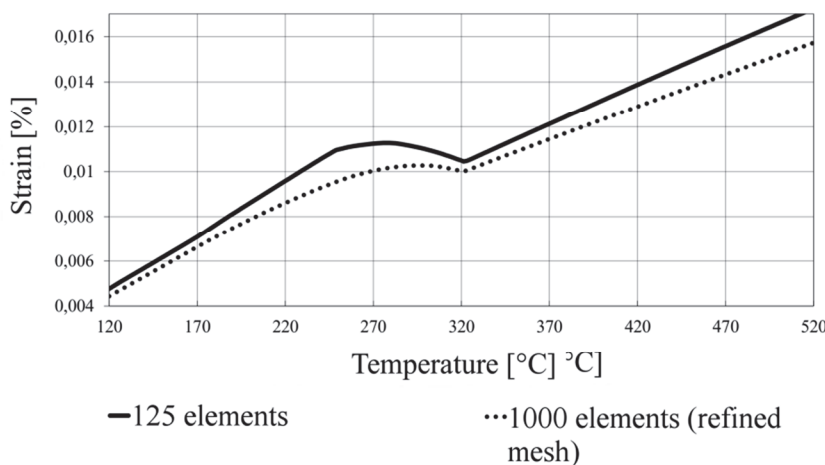
Fig. 8. Dilatometric contraction curves predicted at node 216 for the cooling rate of 5 [°C/s] assuming different mesh refinement of the section and discrete phase transformation.
