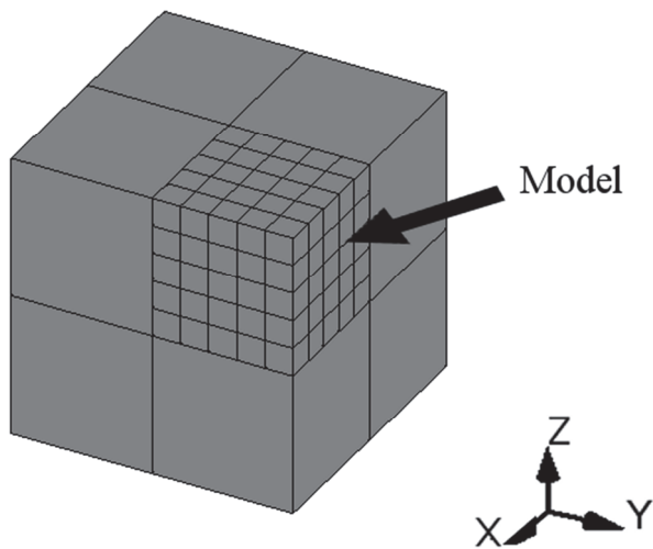
Fig. 3. Schematic representation of the position of the modeled part in the whole element after application of the symmetry planes.
